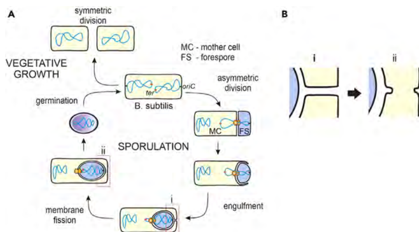
Figure 1. Membrane fission during B. subtilis endospore formation
