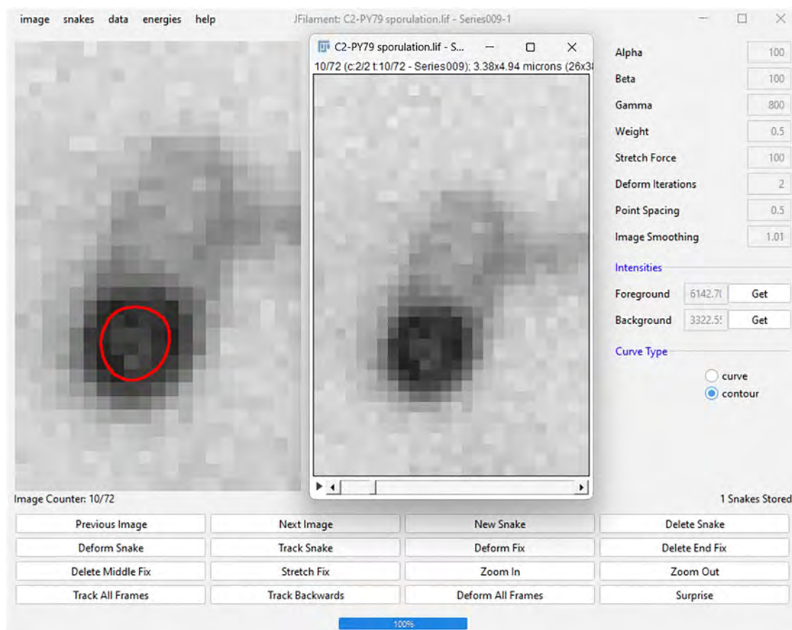
Figure 4. Representative example of fitting a snake to a forespore in JFilament
