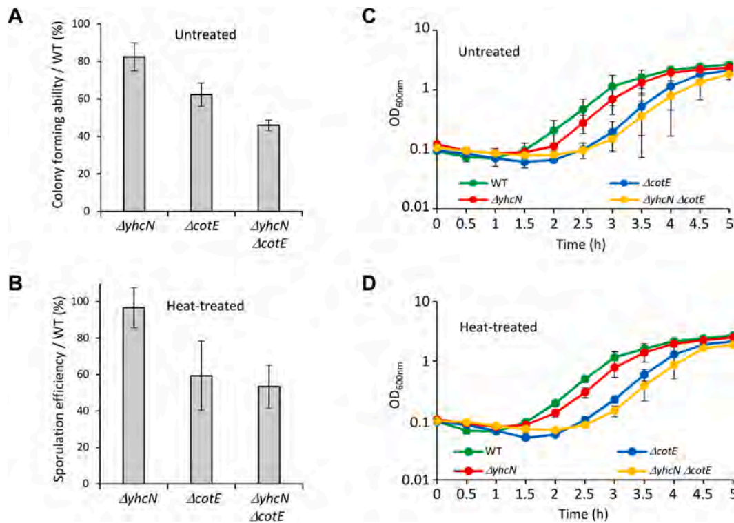
Fig. 2. YhcN is mildly involved in spore outgrowth and colony formation. A-B. Average colony-forming ability of spores ( \pm STDEV, n = 3) (A) or sporulation efficiency ( \pm STDEV, n = 3) (B) of \Delta yhcN (bHC120), \Delta cotE (bHC77) and \Delta yhcN \Delta cotE (bHC126) cells relative to wild-type cells (bDR2413). For colony-forming ability assays (A), purified spores were plated onto solid medium without heat treatment. For sporulation efficiency assays (B), spores were collected 24 h after the onset of sporulation and were treated at 80 °C for 20 min prior to plating onto solid medium. C-D. Average outgrowth time-course ( \pm STDEV, n = 2) of untreated (C) and heat-treated (D) wild-type (WT, bDR2413, green curve), \Delta yhcN (bHC120, red curve), \Delta cotE (bHC77, blue curve) and \Delta yhcN \Delta cotE (bHC126, yellow curve) spores in nutrient-rich medium (LB), monitored by measuring the optical density at 600 nm ( OD_{600nm} ). Optical density first decreases during spore germination and then increases during outgrowth and vegetative growth.
